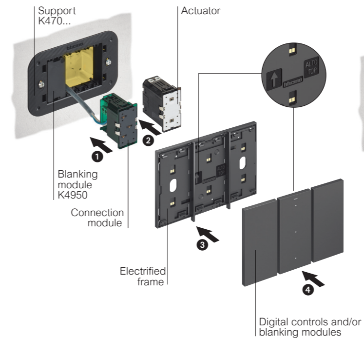
Installation with flush-mounted actuator
