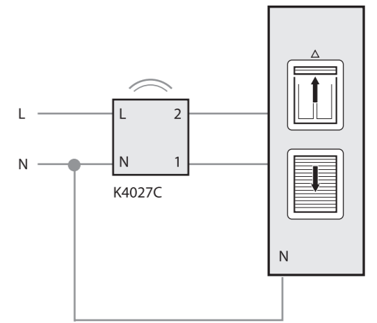
Wiring diagram - interrupted
