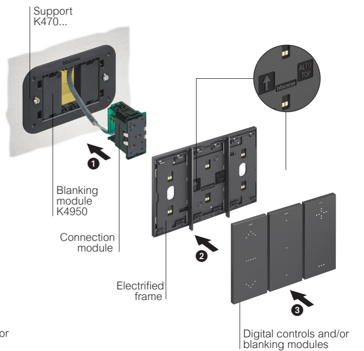
Installation with actuator in DIN switchboard
